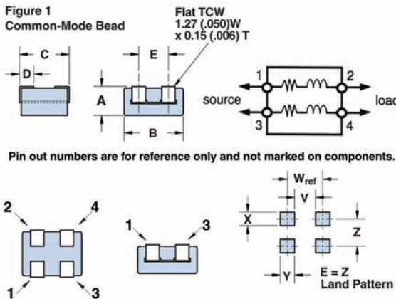
Figure 2 Common-Mode Bead
