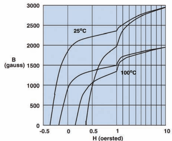
Hysteresis Loop
