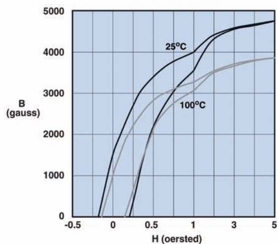
Hysteresis Loop
